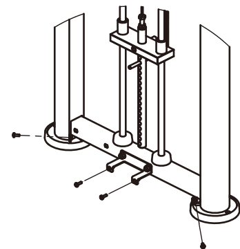
Half Rear Shroud one Bottom Bracket ASSY
