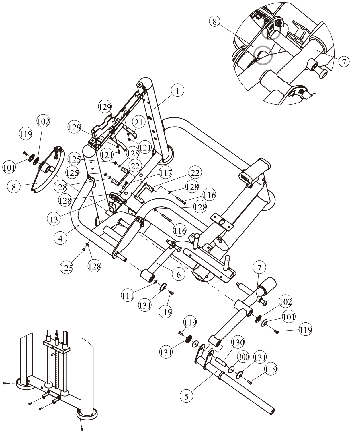
Half Rear Shroud one Bottom Bracket ASSY
